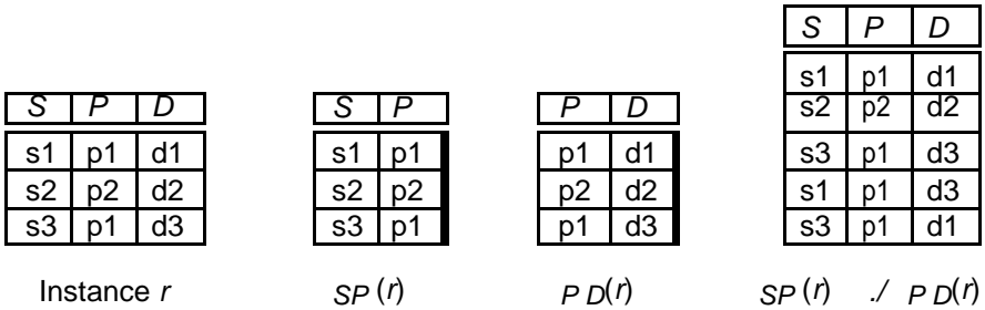
Instances Illustrating Lossy Decompositions
